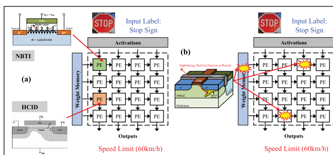
Figure 16. Effects of reliability threats, i.e., (a) aging and (b) soft errors on ML systems.
